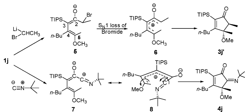
SCHEME 1. Proposed Mechanism for [4+1] of 1j
